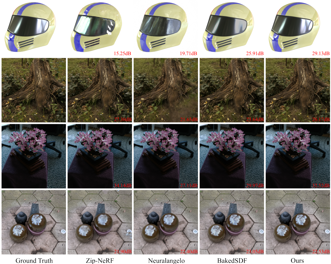
Figure 9: Qualitative comparison with state-of-the-art methods [21, 51, 4] on Shiny Blender [44], Mip-NeRF 360 [3] and Ref-NeRF real [44] datasets. PSNR values for each image patch are inset. Best viewed when zoomed in.
