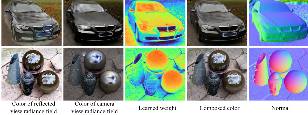
Figure 3: Visualization of the color of reflected view radiance field, color of camera view radiance field, learned weight \mathbf{W} , composed color and surface normal on “sedan” and “garden spheres” scenes [44]. Our method assigns high weight (red color) for reflective surfaces, e.g. , window and hood of sedan, spheres, without any supervision.
